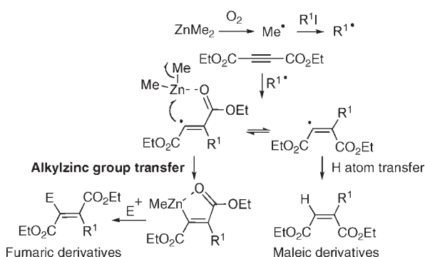
Scheme 2. Proposed Mechanism
